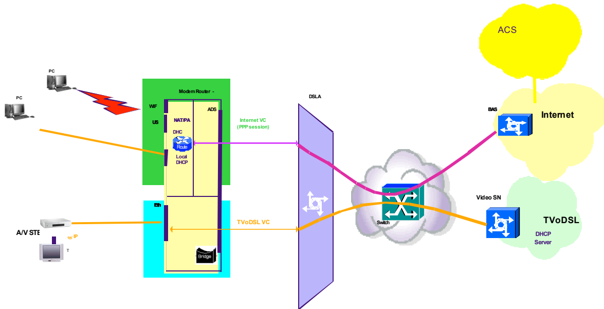
Figure 3 – Example of interface-based bridging
