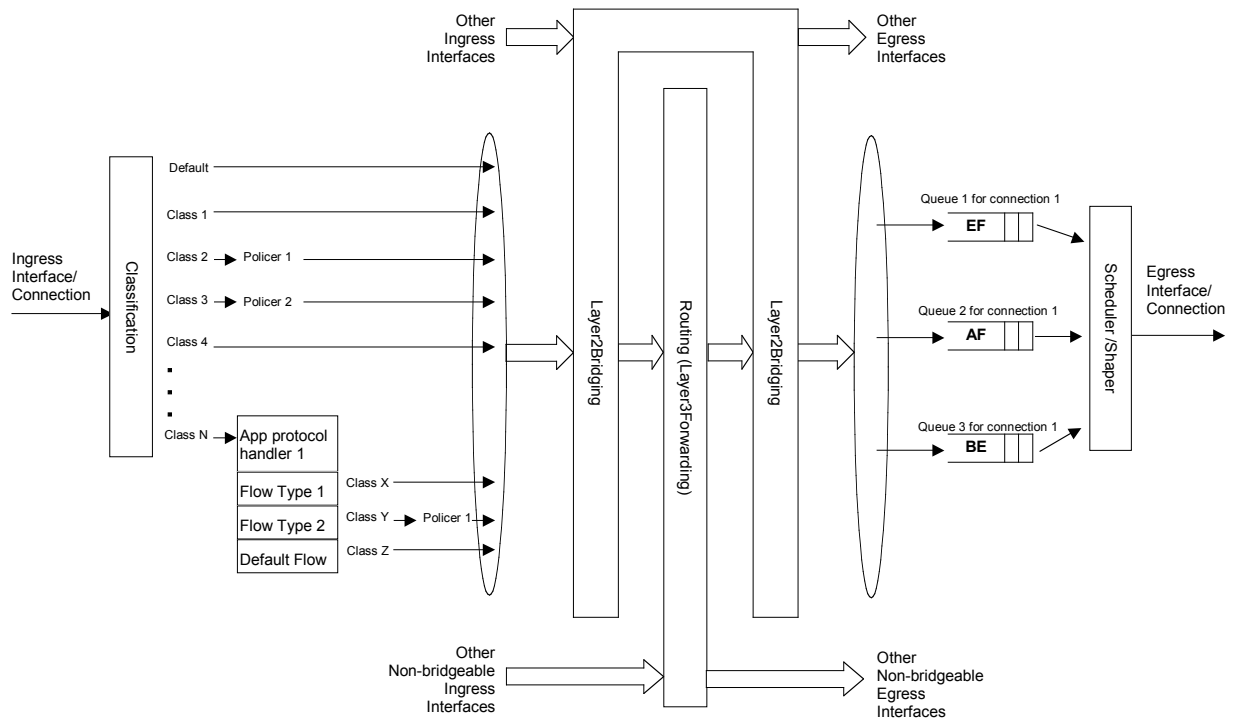
Figure 1 – Queuing model of an Internet Gateway Device
