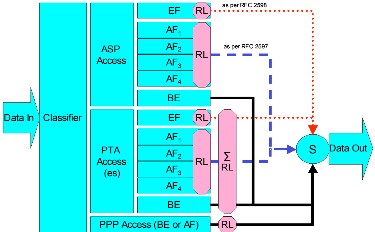
Figure 2 – Queuing and Scheduling Example for RG
